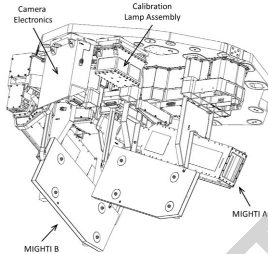
Figure 3: Isometric view of the MIGHTI instrument integrated on the ICON Payload Interface Plate (PIP). In this view the zenith direction is up and the MIGHTI sensors are pointed downward at the Earth's limb.
