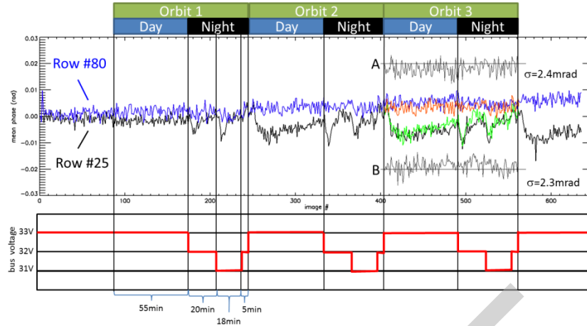
Figure 19: Top panel: Black, blue: Mean phase versus image number for two rows (25 and 80, respectively), which correspond to tangent altitudes of approximately 300km and 150km (top and bottom of red fringes, MIGHTI B, red-line). Red, green: Phase data from simulated Orbit 2 shifted to line up with Orbit 3 for comparison. A, B: Difference of red-blue and green-black, shifted up and down for clarity. Horizontal lines show zero difference. Bottom panel: Corresponding bus voltage versus image number. Integration time was 30s, interval between images was about 7.6 sec (Ground support equipment (GSE) read out time). No dark, flatfield, or spike correction was performed for this analysis.
