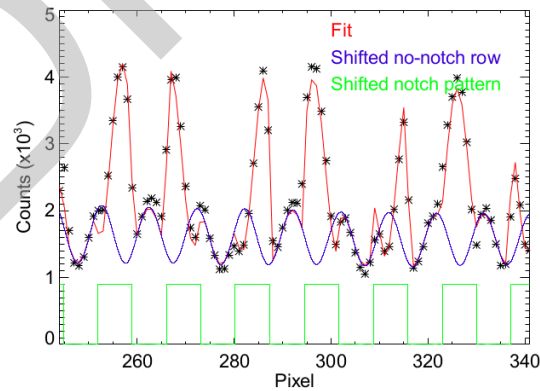
Figure 17: Locating the horizontal notch pattern position. The stars indicate the measured values (Ne calibration lamp) for a pixel row containing the notch pattern. The blue curve indicates a scaled and phase shifted fringe pattern from a pixel row just below the notch pattern to optimally fit the pixels that fall inside the notches. For the pixels that fall outside the notches, an analogous fringe pattern is obtained by scaling and phase shifting the same fringe pattern from below the
