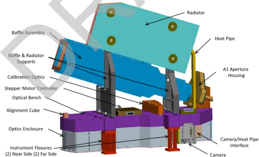
Figure 4: A single MIGHTI sensor unit.
