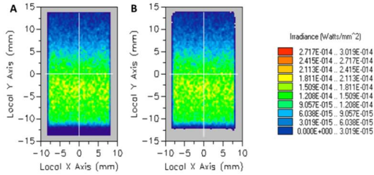
Figure 8: Results for scattered light calculation from the illuminated Earth's disk at 630nm. The images show the flux at the interferometer gratings. (A) All rays; (B) direct rays only, no ghosts, no scatter. Integrated flux: All rays: 4.490 \times 10^{-12} \text{ W} ; Direct rays: 4.436 \times 10^{-12} \text{ W} . Ghosts plus scatter amount to 5.4 \times 10^{-14} \text{ W} or 1.2% of the direct signal
