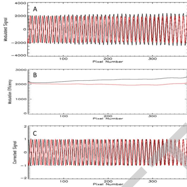
Figure 16: (A) Modulated part of a responsivity- and dark-corrected interferogram measured using the external integrating sphere illuminated with a neon lamp. Two binned pixel CCD rows near the top and the bottom of the altitude range are shown for MIGHTI A in night mode to illustrate row to row differences in the modulation efficiency. Signal is in arbitrary units. (B) Calculated modulation efficiency for the two rows in (A). (C) Modulation efficiency corrected fringe patterns for the two rows shown in (A). Note that the fringe amplitude after the correction is now constant (normalized) and equal for both.
