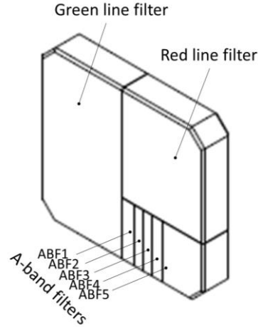
Figure 11: Mosaic filter geometry.
