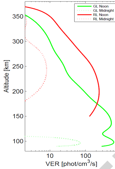
Figure 1: Volume emission rates of the oxygen green (GL) and red (RL) line emissions used for the MIGHTI instrument model.
