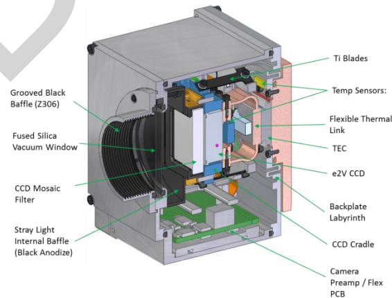
Figure 13: MIGHTI camera head cut-away.
