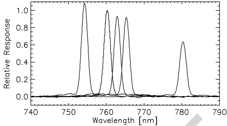
Figure 15: Spectral response within the areas of all five NIR filters. Each curve represents an average spectral response of 36 binned pixels in one CCD row at approximately the center altitude covered by the filters. The response shape is dominated by the passband of the narrow band filters. The three passbands in the middle are within the oxygen A-band, the remaining two are used to perform a background signal subtraction [Stevens et al. 2016].
