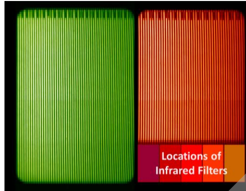
Figure 12: False color image of calibration lamp signal taken with MIGHTI A. This image is binned by 2 pixels in the vertical and 2 pixels in the horizontal dimension. On orbit, the binning will be 16 \times 2 (vertical \times horizontal) and the vertical dimension will cover the tangent point altitudes between about 90-300km. The top of both red and green images show the periodic notch pattern that is inscribed onto one of the gratings of each interferometer. This pattern is used to track any residual horizontal image shifts on the CCD detector [Englert et al. 2010b]. The locations of the NIR filters are shown on the bottom right using superimposed rectangles as they are not illuminated by the calibration lamps.
