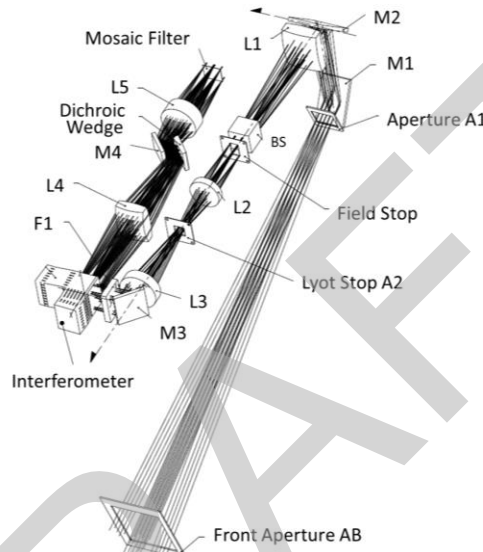
Figure 10: MIGHTI optical components shown with representative rays.
