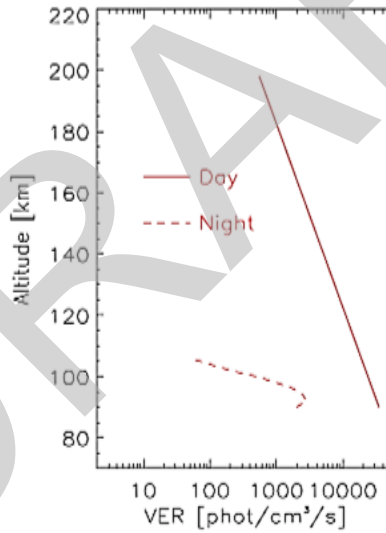
Figure 2: Average volume emission rates of the oxygen A-band used for the MIGHTI instrument model.
